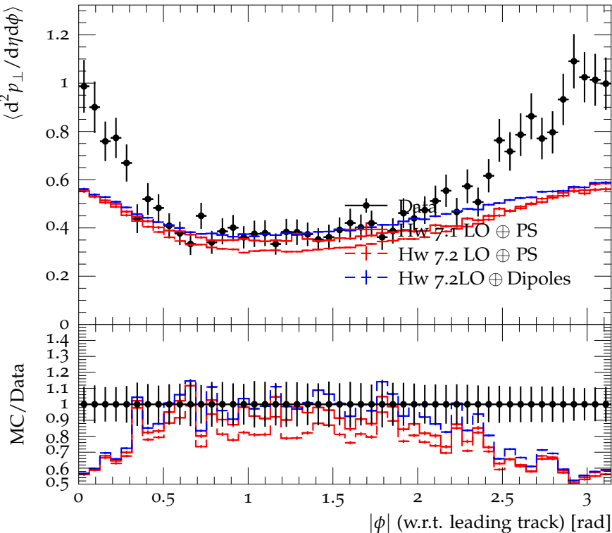
p_{\perp} density vs. \Delta\phi , p_{\perp}^{\text{trk1}} > 2.5 GeV, \sqrt{s} = 900 GeV
