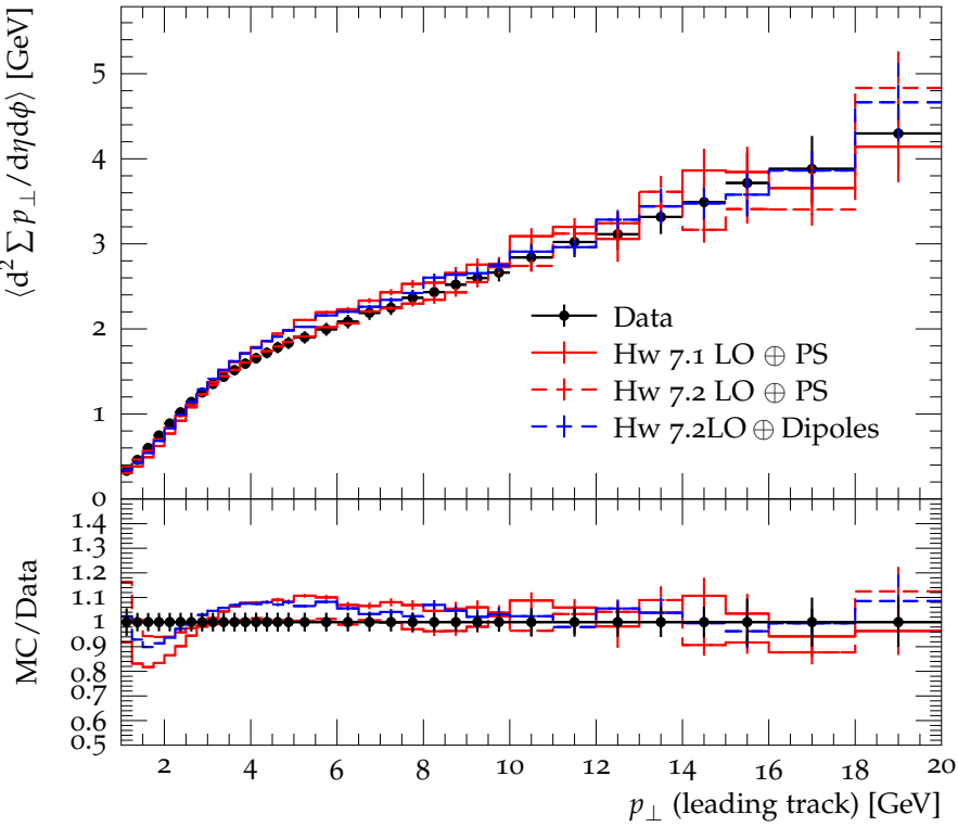
Toward \Sigma p_{\perp} density vs. p_{\perp}^{\text{trk1}} , \sqrt{s} = 7 TeV, p_{\perp} > 100 MeV
