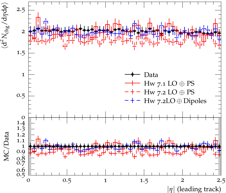
Transverse N_{\text{chg}} density vs. |\eta^{\text{trk1}}| , \sqrt{s} = 7 TeV, p_{\perp} > 100 MeV
