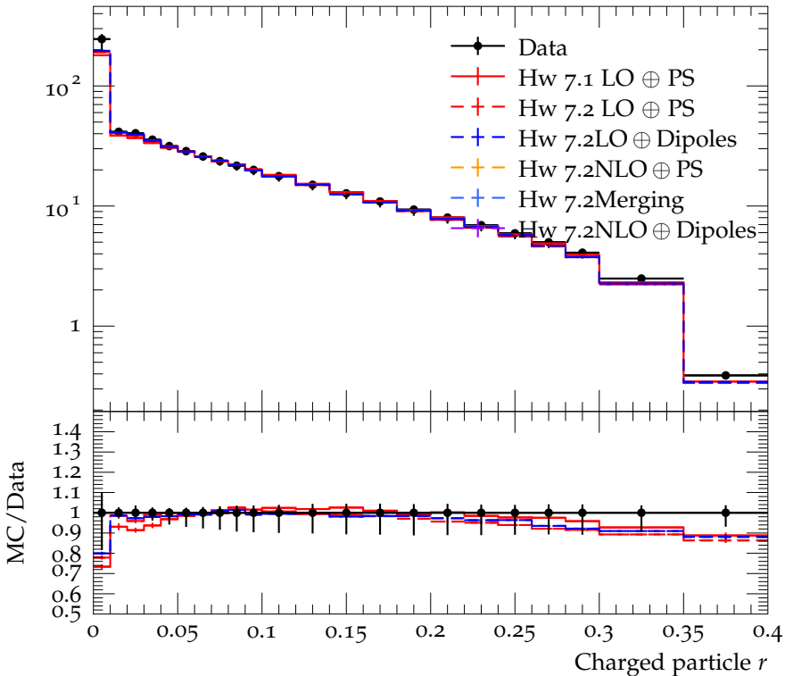
Charged jet \rho_{\text{ch}}(r) (anti- k_t , R = 0.4 , y 0.0-1.9, p_{\perp} 4.0-6.0)
