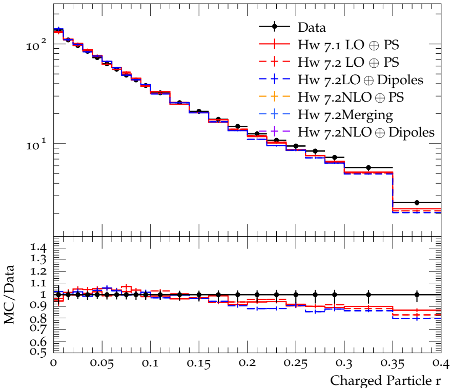
Charged jet \rho_{\text{ch}}(r) (anti- k_t , R = 0.4 , y 0.0-1.9, p_{\perp} 15.0-24.0)
