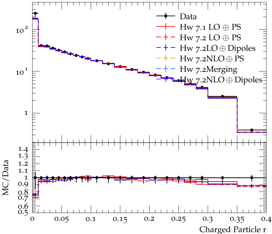
Charged jet \rho_{\text{ch}}(r) (anti- k_t , R = 0.4 , y 0.0-0.5, p_{\perp} 4.0-6.0)
