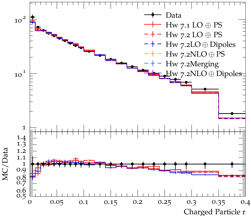
Charged jet \rho_{\text{ch}}(r) (anti- k_t , R = 0.4 , y 0.5-1.0, p_{\perp} 10.0-15.0)
