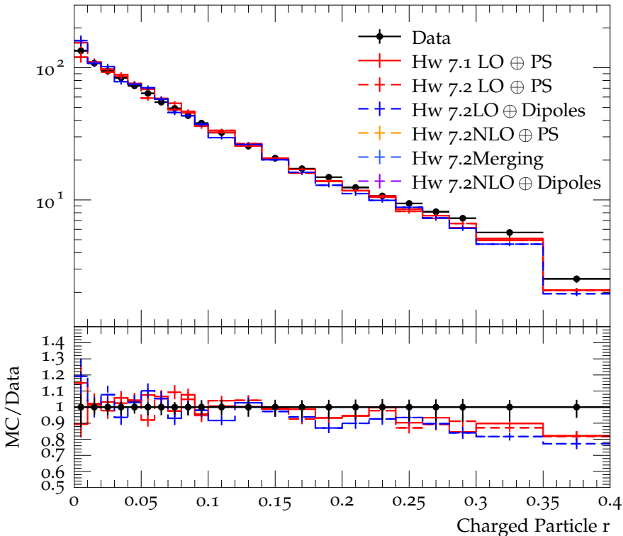
Charged jet \rho_{\text{ch}}(r) (anti- k_t , R = 0.4 , y 1.0-1.5, p_{\perp} 15.0-24.0)
