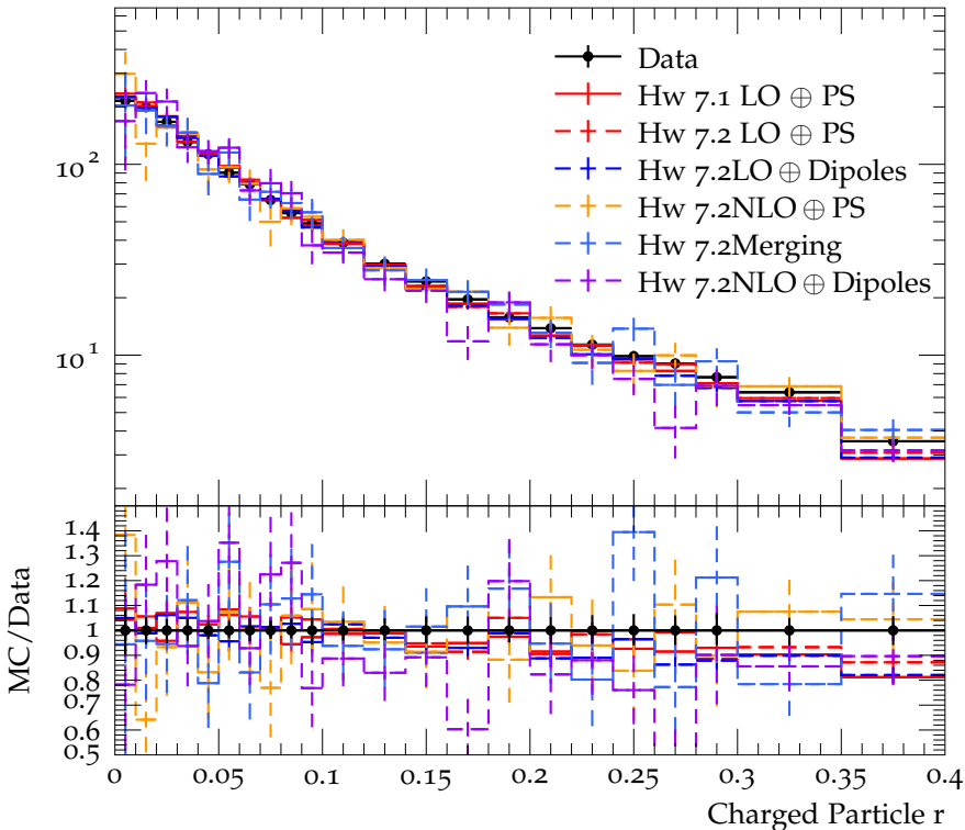
Charged jet \rho_{\text{ch}}(r) (anti- k_t , R = 0.4 , y 1.0-1.5, p_{\perp} 24.0-40.0)
