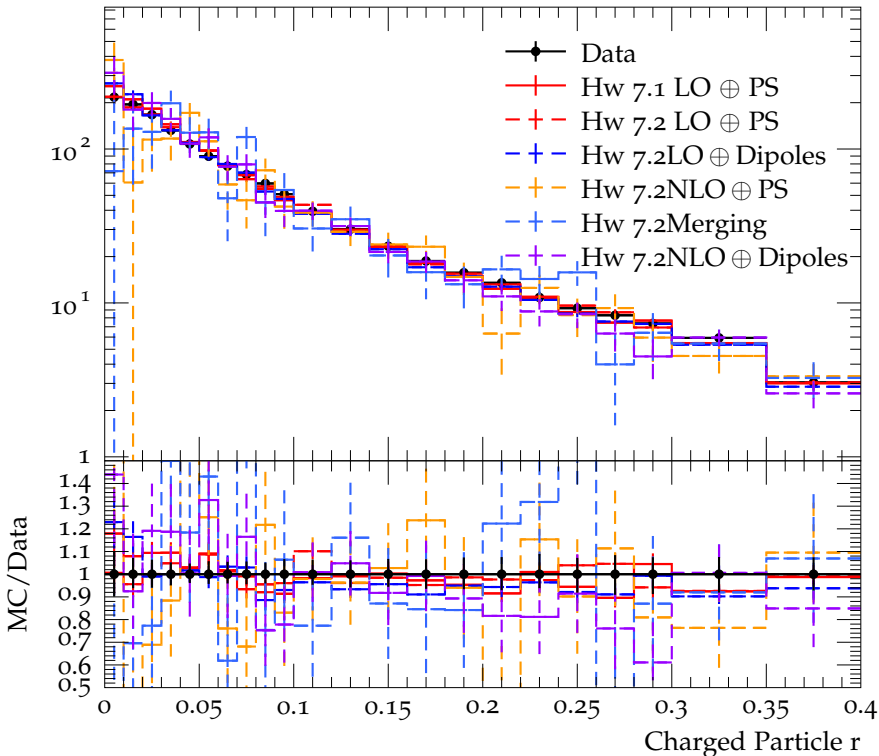
Charged jet \rho_{\text{ch}}(r) (anti- k_t , R = 0.4 , y 1.5-1.9, p_{\perp} 24.0-40.0)
