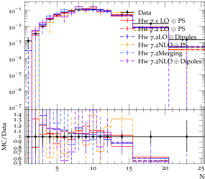
Charged jet multiplicity (anti- k_t , R = 0.6 , y 0.5-1.0, p_\perp 24.0-40.0)
