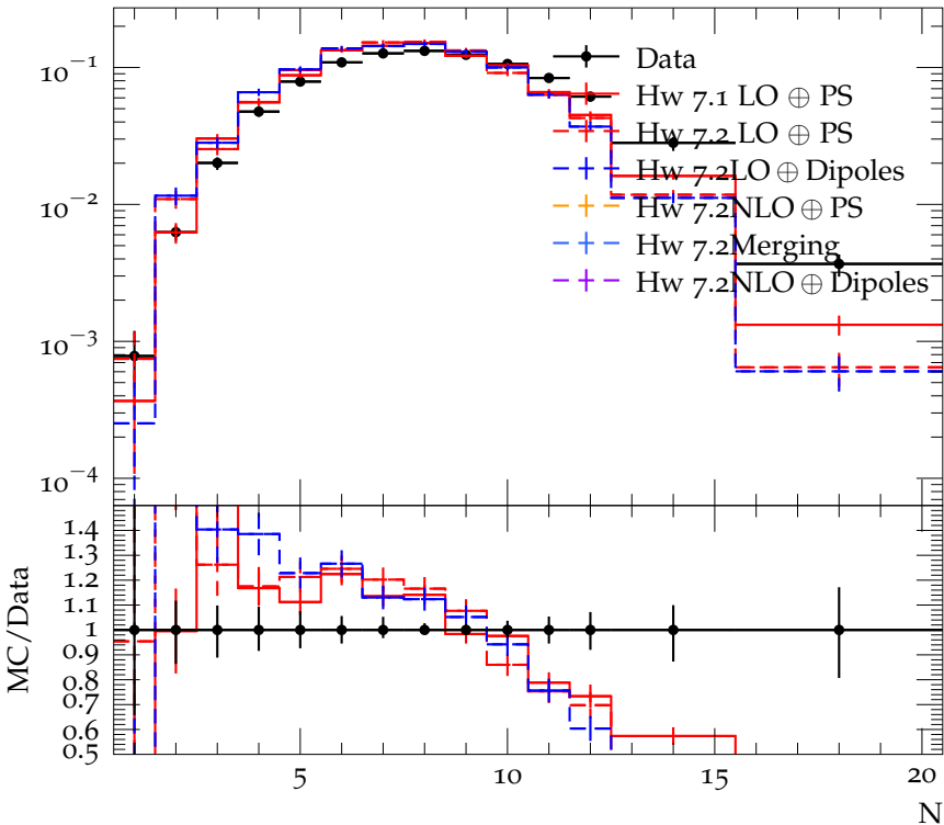
Charged jet multiplicity (anti- k_t , R = 0.6 , y 1.0-1.5, p_\perp 15.0-24.0)
