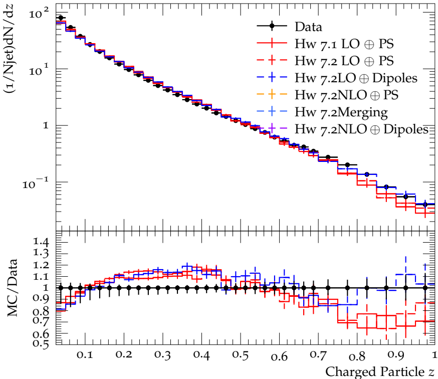
Charged jet z (anti- k_t , R = 0.6 , y 0.0-1.9, p_\perp 15.0-24.0)
