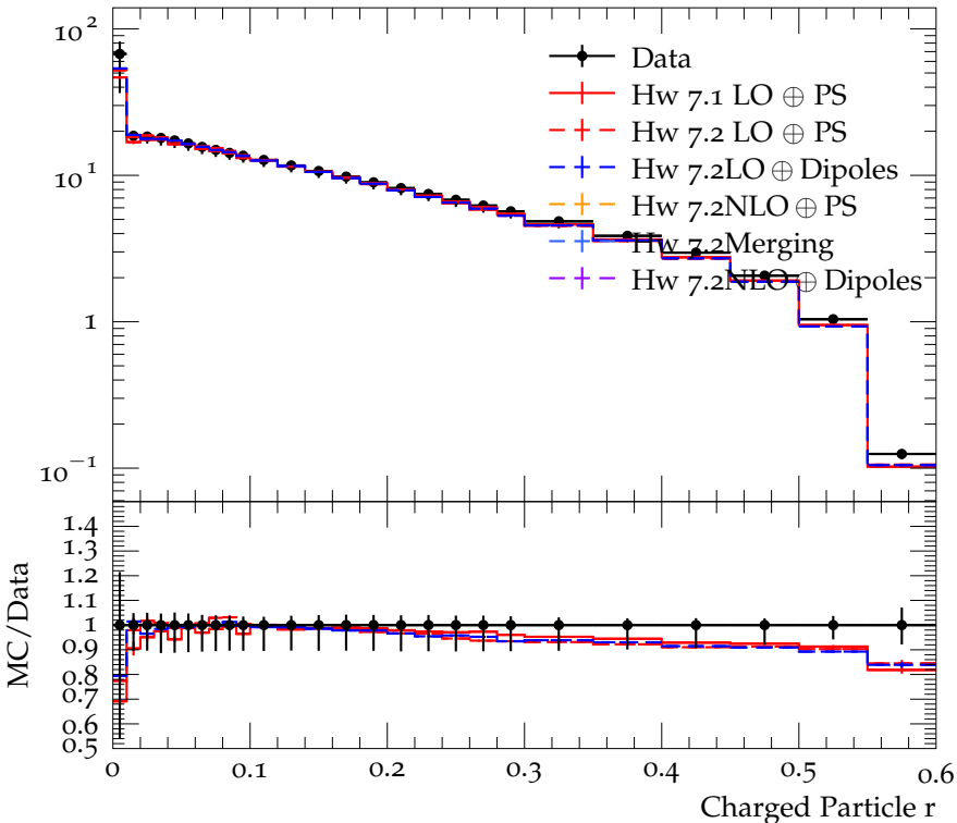
Charged jet \rho_{\text{ch}}(r) (anti- k_t , R = 0.6 , y 0.0-1.9, p_{\perp} 4.0-6.0)
