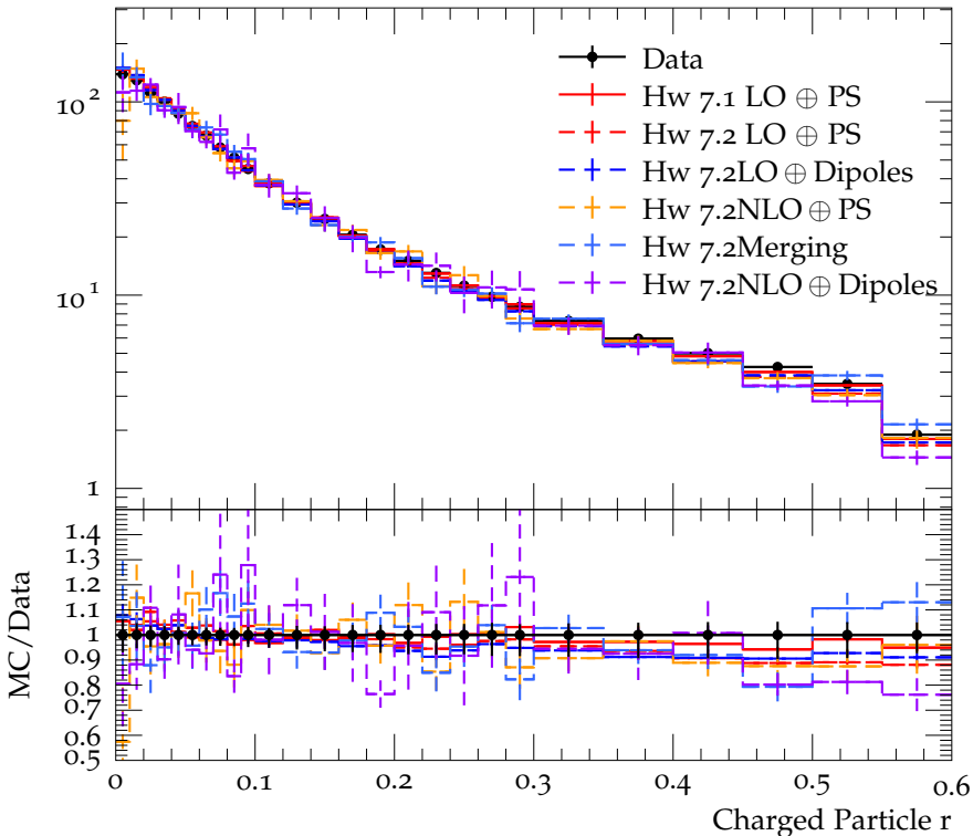
Charged jet \rho_{\text{ch}}(r) (anti- k_t , R = 0.6 , y 0.0-1.9, p_{\perp} 24.0-40.0)
