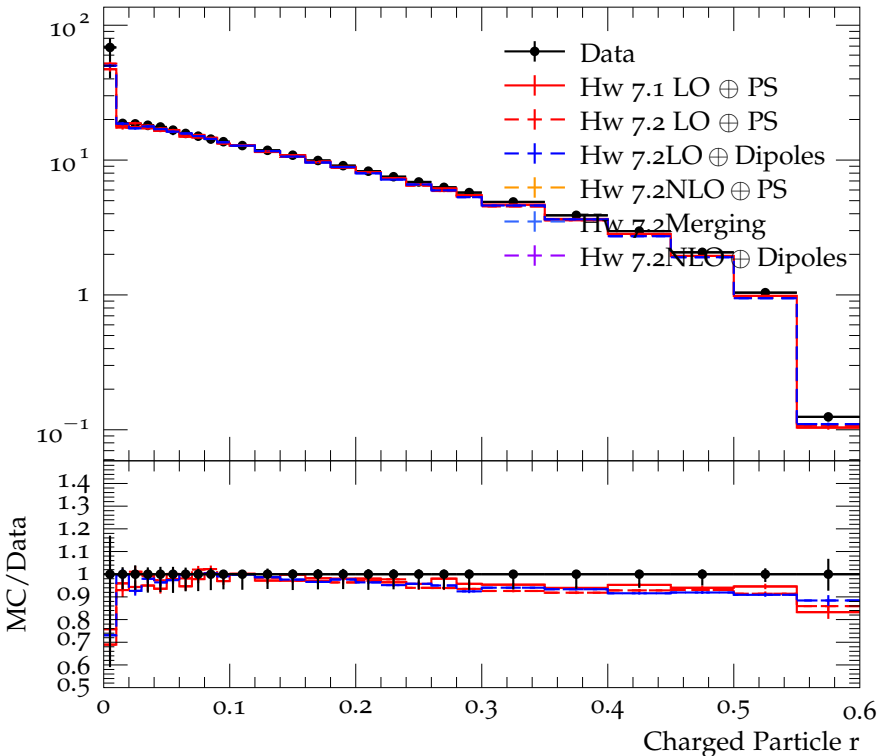
Charged jet \rho_{\text{ch}}(r) (anti- k_t , R = 0.6 , y 0.0-0.5, p_{\perp} 4.0-6.0)
