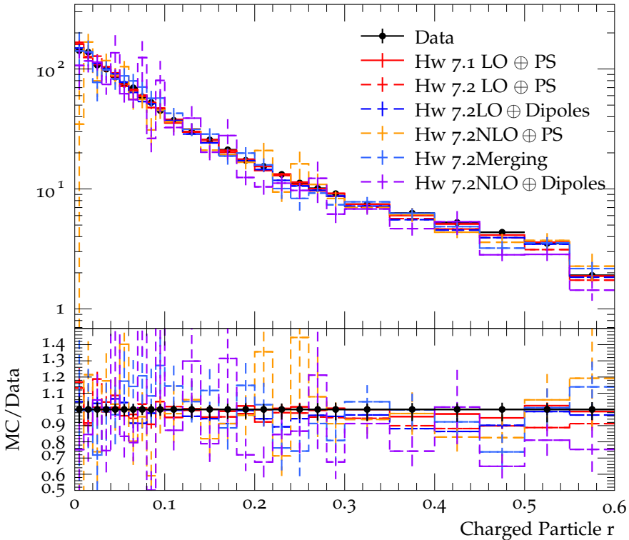
Charged jet \rho_{\text{ch}}(r) (anti- k_t , R = 0.6 , y 0.0-0.5, p_{\perp} 24.0-40.0)
