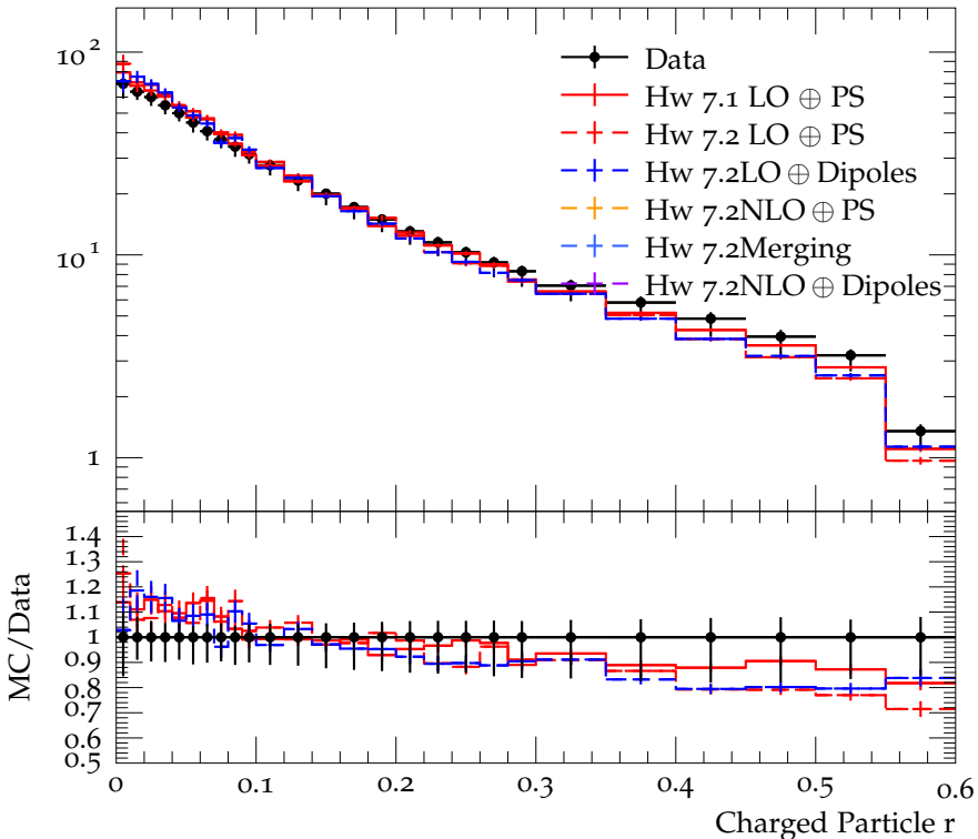
Charged jet \rho_{\text{ch}}(r) (anti- k_t , R = 0.6 , y 1.5-1.9, p_{\perp} 15.0-24.0)
