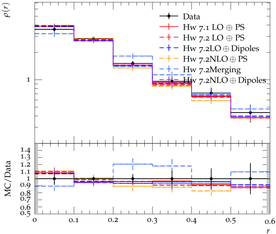
Jet shape \rho for p_{\perp} \in 30\text{--}40\text{GeV} , y \in 2.1\text{--}2.8
