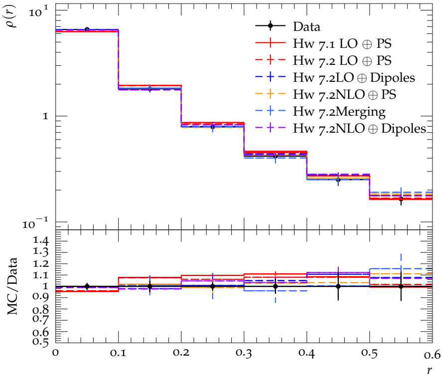
Jet shape \rho for p_{\perp} \in 160\text{--}210\text{ GeV} , y \in 0.0\text{--}0.3
