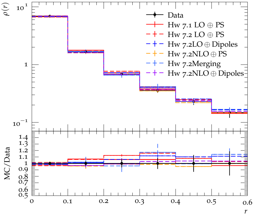
Jet shape \rho for p_{\perp} \in 160\text{--}210\text{GeV} , y \in 1.2\text{--}2.1
