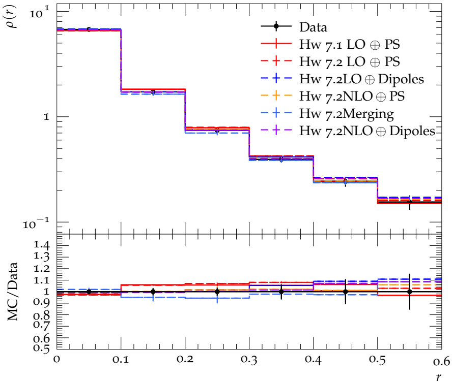
Jet shape \rho for p_{\perp} \in 160\text{--}210\text{ GeV} , y \in 0.0\text{--}2.8
