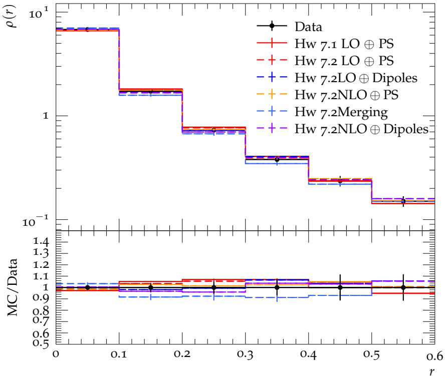
Jet shape \rho for p_{\perp} \in 210\text{--}260\text{ GeV} , y \in 0.0\text{--}0.3
