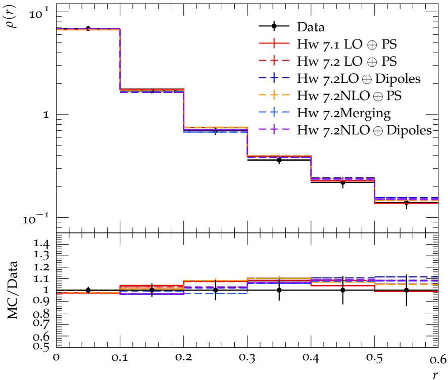
Jet shape \rho for p_{\perp} \in 210\text{--}260\text{ GeV} , y \in 0.3\text{--}0.8
