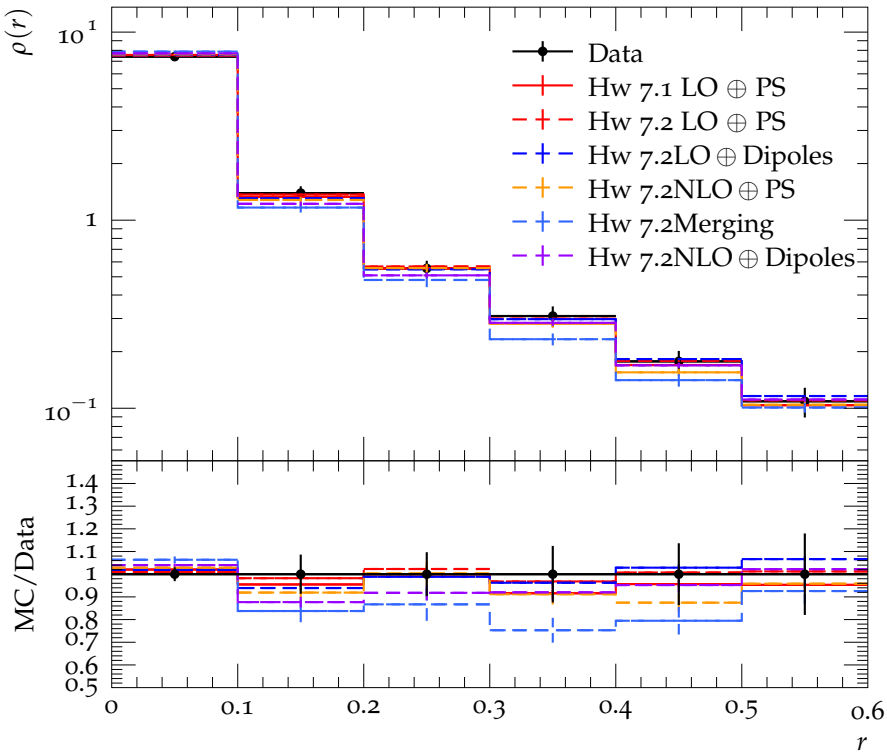
Jet shape \rho for p_{\perp} \in 210\text{--}260\text{ GeV} , y \in 2.1\text{--}2.8
