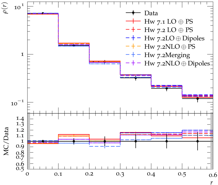
Jet shape \rho for p_{\perp} \in 260\text{--}310\text{ GeV} , y \in 0.0\text{--}0.3
