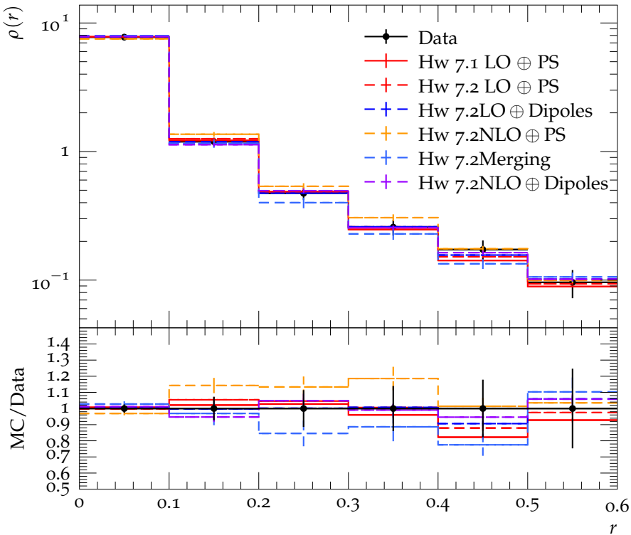
Jet shape \rho for p_{\perp} \in 260\text{--}310\text{GeV} , y \in 2.1\text{--}2.8
