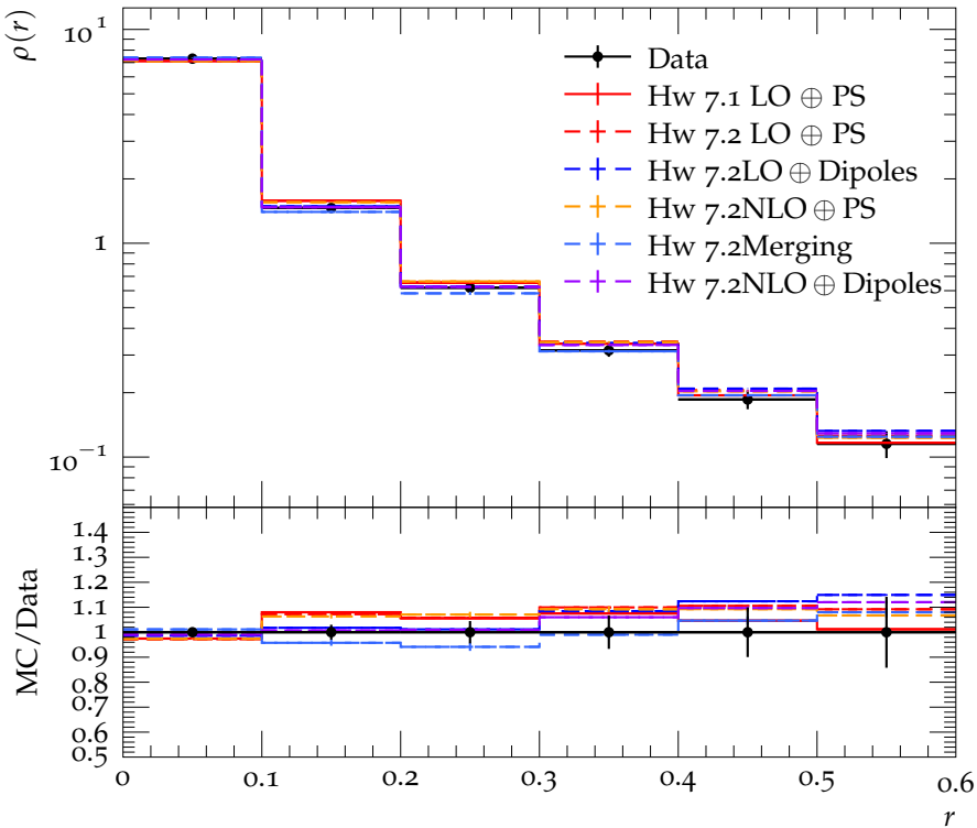
Jet shape \rho for p_{\perp} \in 260\text{--}310\text{ GeV} , y \in 0.0\text{--}2.8
