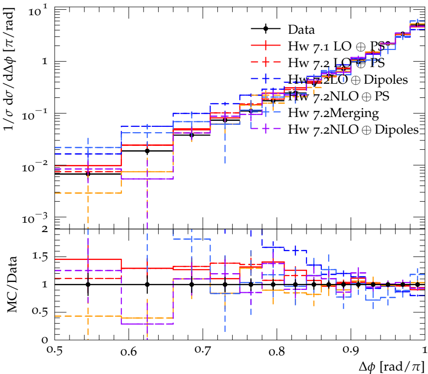
Dijet azimuthal decorrelations for 110 < p_{\perp}^{\max}/\text{GeV} < 160
