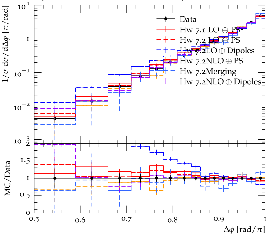
Dijet azimuthal decorrelations for 210 < p_{\perp}^{\text{max}}/\text{GeV} < 260
