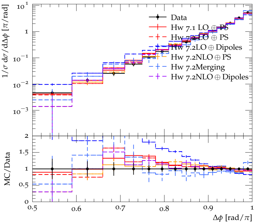
Dijet azimuthal decorrelations for 260 < p_{\perp}^{\text{max}}/\text{GeV} < 310
