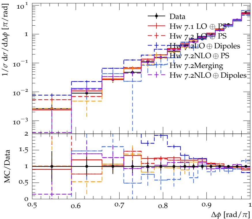
Dijet azimuthal decorrelations for 310 < p_{\perp}^{\text{max}}/\text{GeV} < 400
