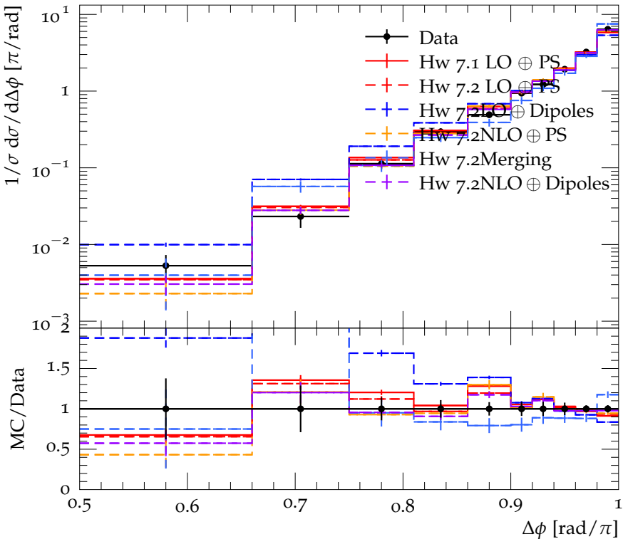
Dijet azimuthal decorrelations for 400 < p_{\perp}^{\max}/\text{GeV} < 500
