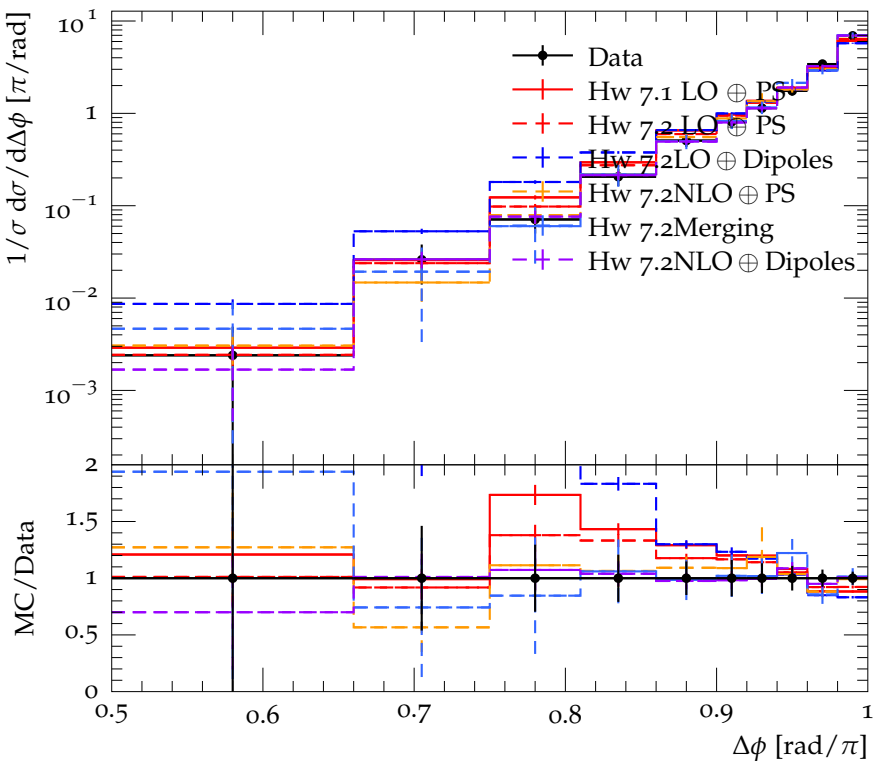
Dijet azimuthal decorrelations for 500 < p_{\perp}^{\text{max}}/\text{GeV} < 600
