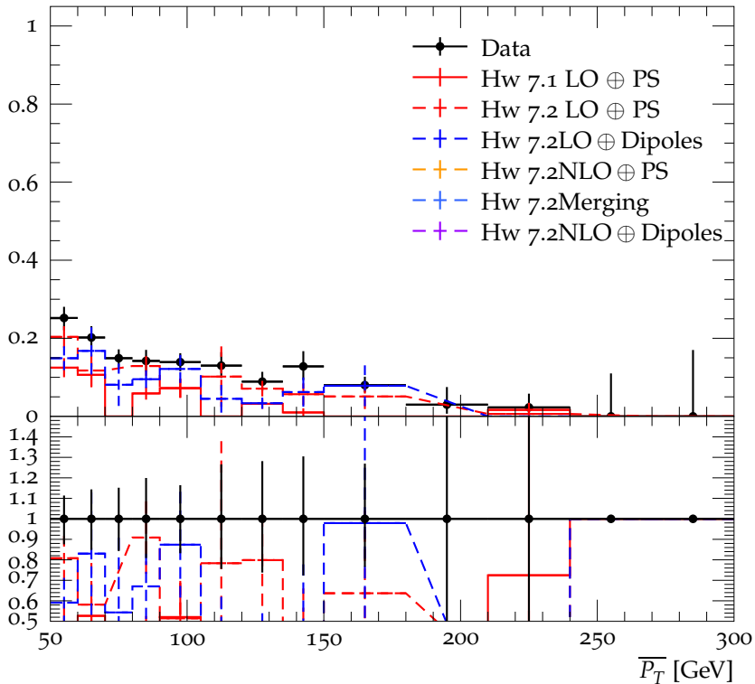
Gap fraction vs \overline{P_T} for 5.0 < |\Delta y| < 6.0 , Fwd/Bwd
