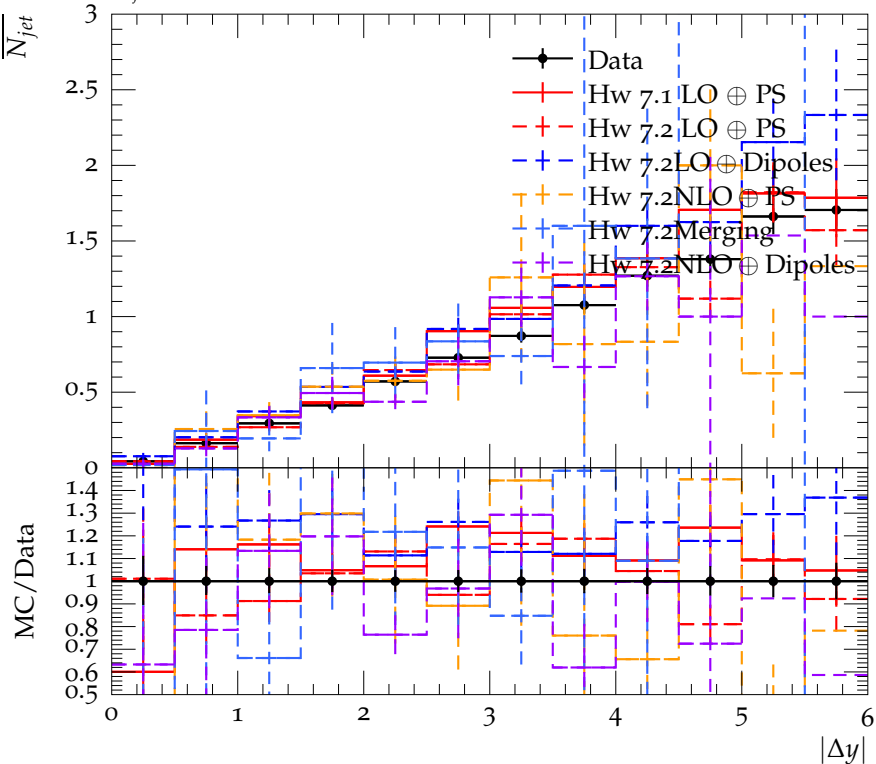
\overline{N}_{jet} vs |\Delta y| for 70 < \overline{P}_T < 90 , Fwd/Bwd
