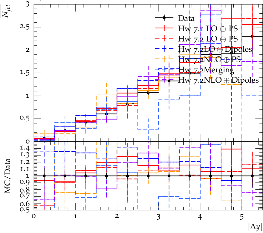
\overline{N}_{jet} vs |\Delta y| for 180 < \overline{P}_T < 210 , Fwd/Bwd
