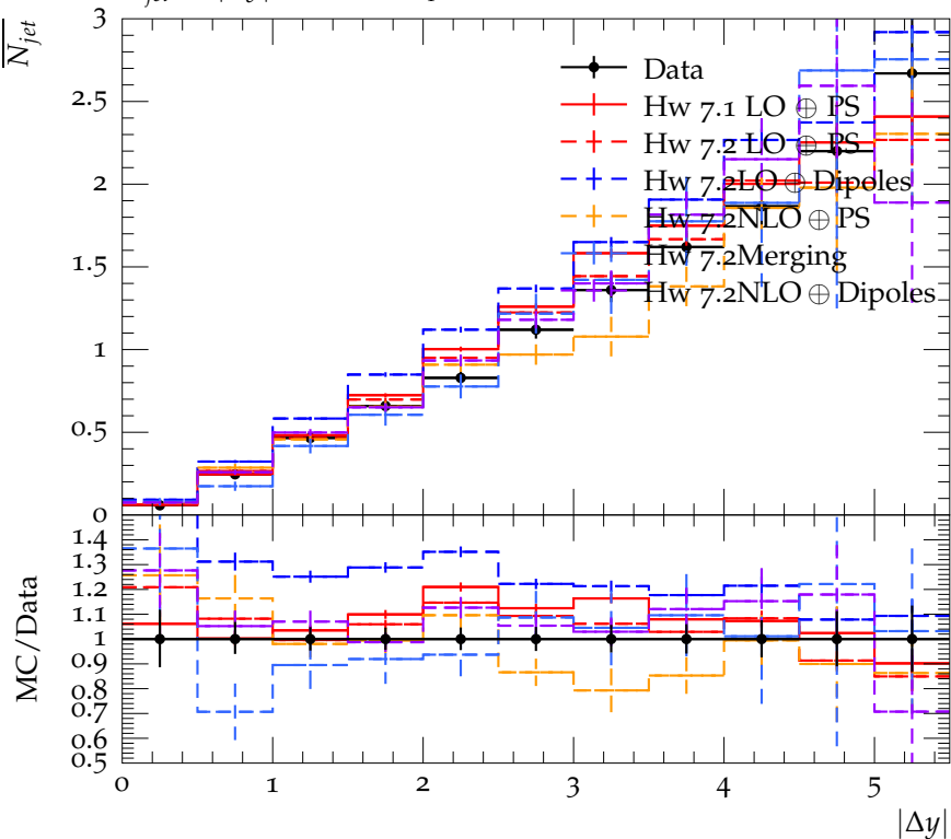
\overline{N}_{jet} vs |\Delta y| for 210 < \overline{P}_T < 240 , Fwd/Bwd
