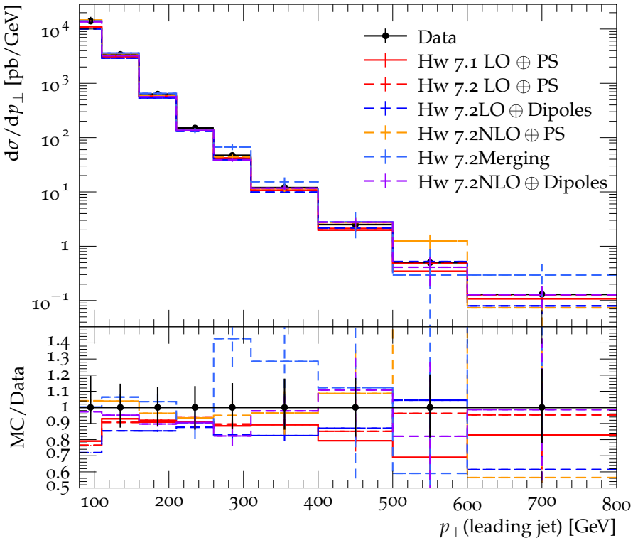
Transverse momentum of the leading jet ( R = 0.4 )
