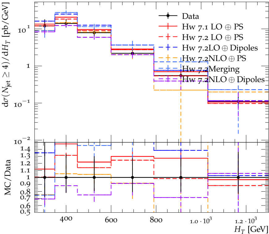
H_T for events with N_{\text{jet}} \geq 4 ( R = 0.4 )
