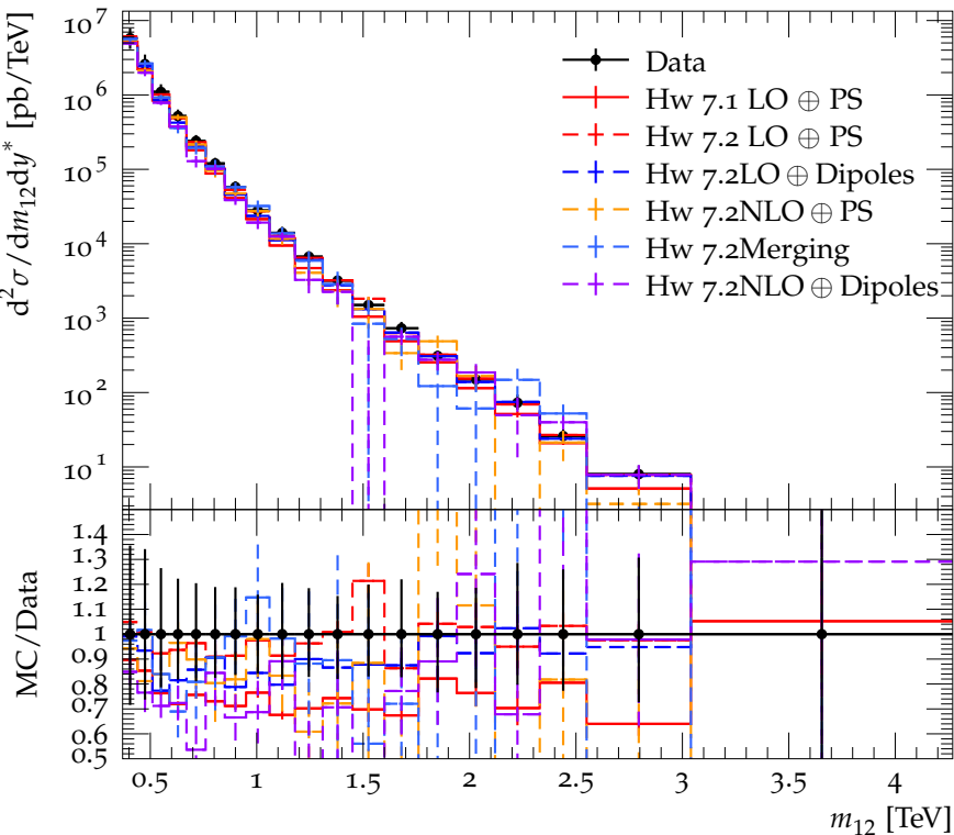
Dijet double-diff. x-section, anti- k_t 0.4 ( 2.0 \leq y^* < 2.5 )
