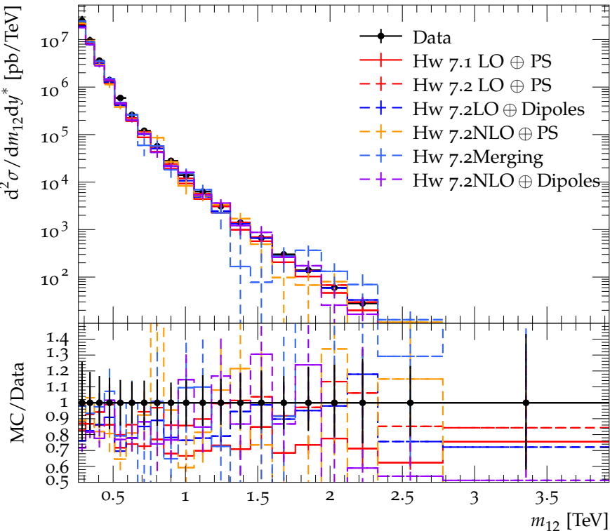
Dijet double-diff. x-section, anti- k_t 0.6 ( 1.5 \leq y^* < 2.0 )
