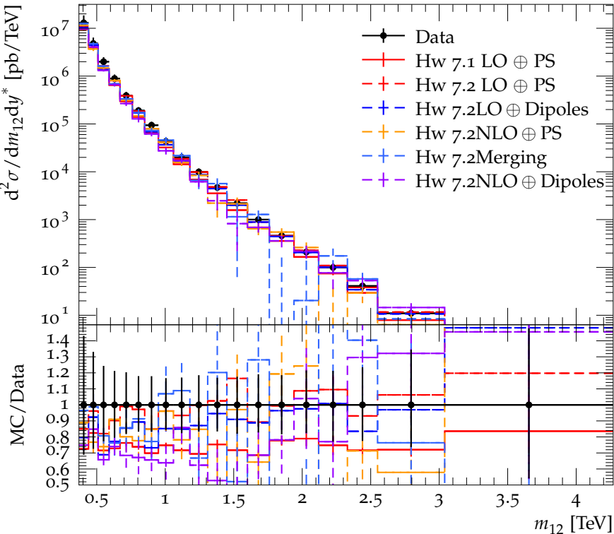
Dijet double-diff. x-section, anti- k_t 0.6 ( 2.0 \leq y^* < 2.5 )
