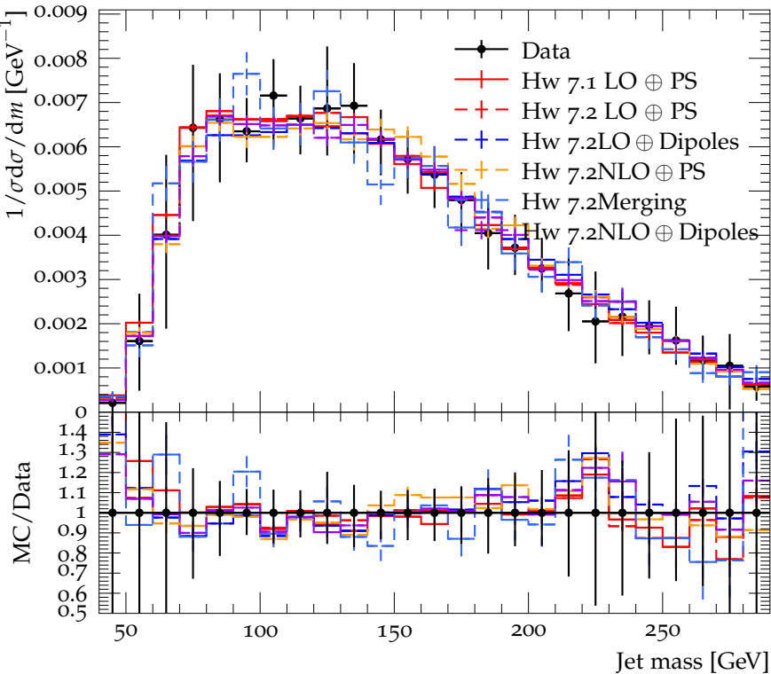
Cambridge-Aachen filtered jets, R=1.2 , 400 \text{ GeV} < p_{\perp} < 500 \text{ GeV}
