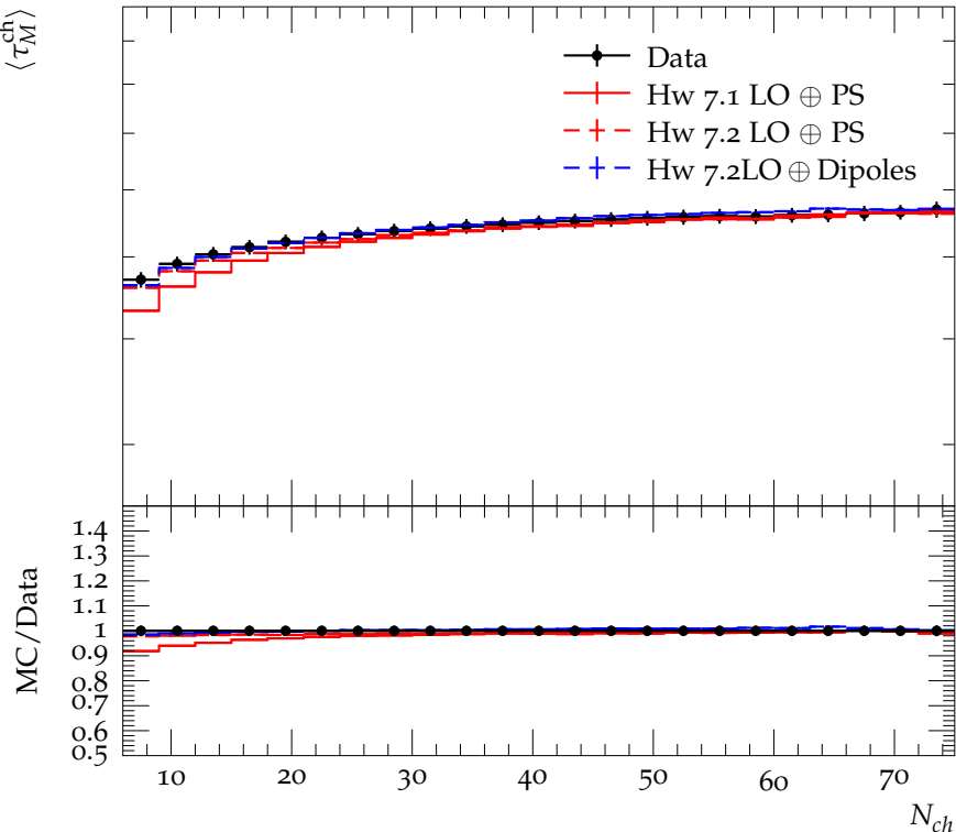
Average transverse thrust minor vs. multiplicity
