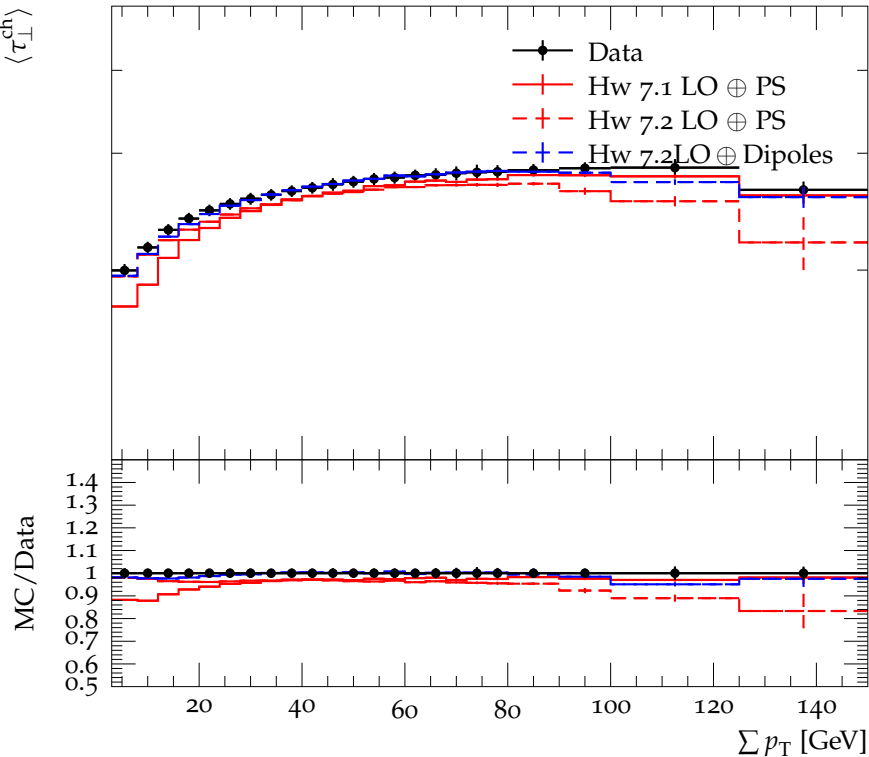
Average transverse thrust vs. transverse \Sigma p_T
