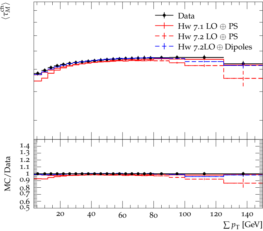
Average transverse thrust minor vs. transverse \Sigma p_T
