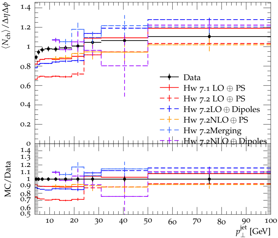
Mean N_{\text{ch}} vs. leading jet p_{\perp} , R = 0.2 , Transverse region
