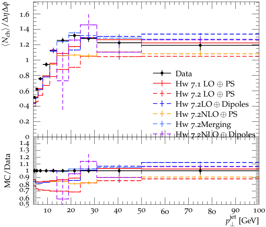
Mean N_{\text{ch}} vs. leading jet p_{\perp} , R = 1.0 , Transverse region
