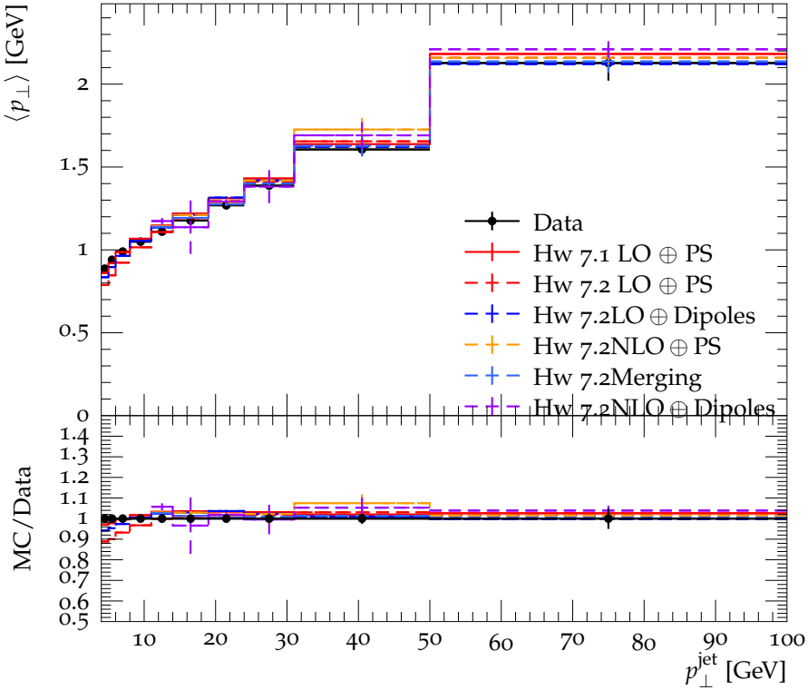
Mean p_{\perp} vs. leading jet p_{\perp} , R = 1.0 , Away region
